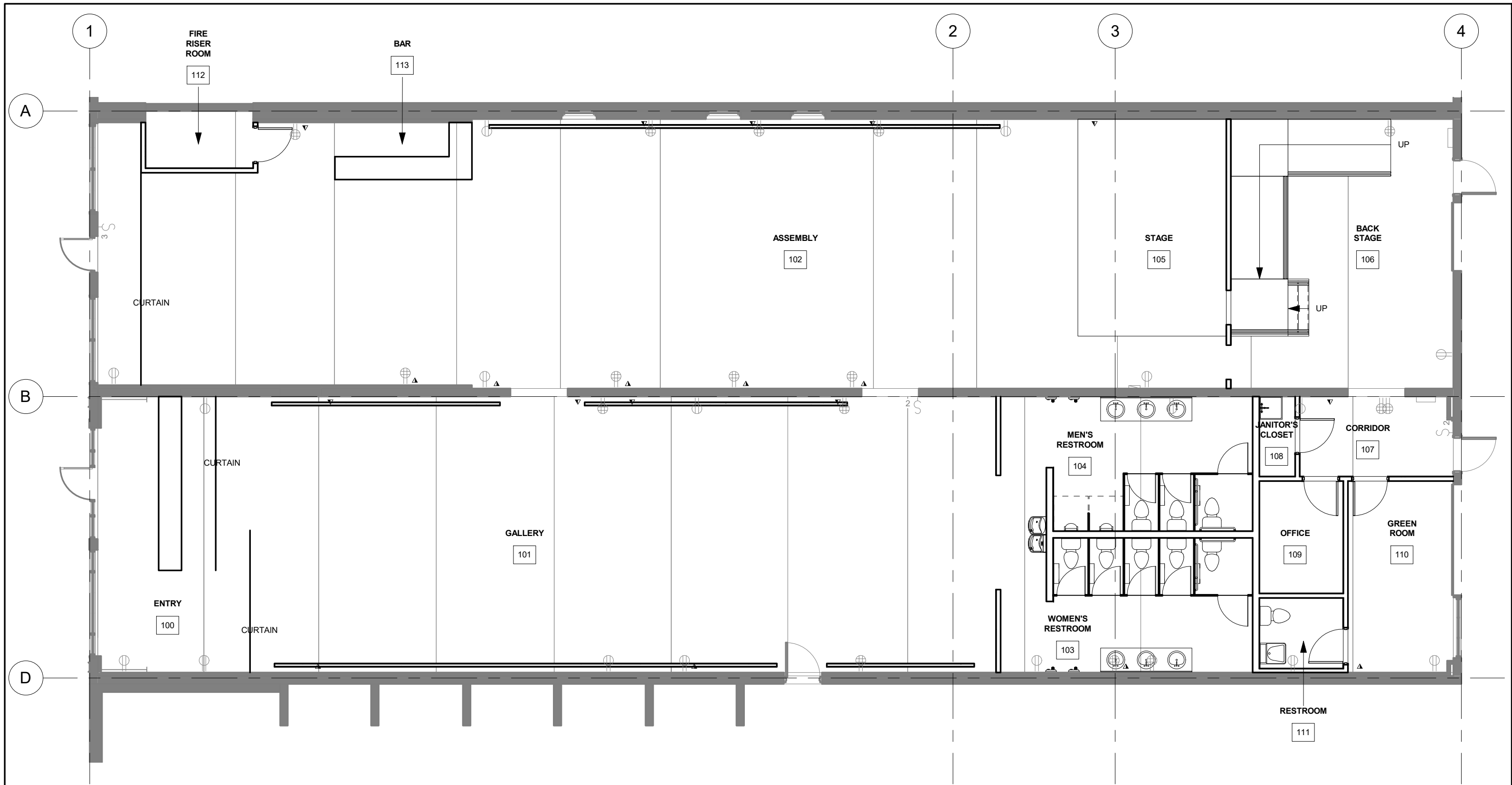
1 FLOOR PLAN A1.0 1/8" = 1'-0"
